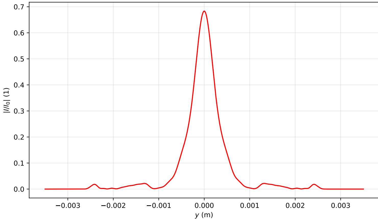
Intensity profile I(x=0, y, z=3.105)/I_0 , P_{in}=3.5P_{cr} , artificial time
